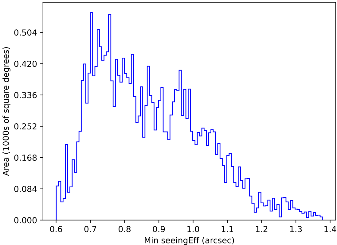
too_elab_r8_d2_giz_v3.4_10yrs Yr 1 u band: Min seeingEff
