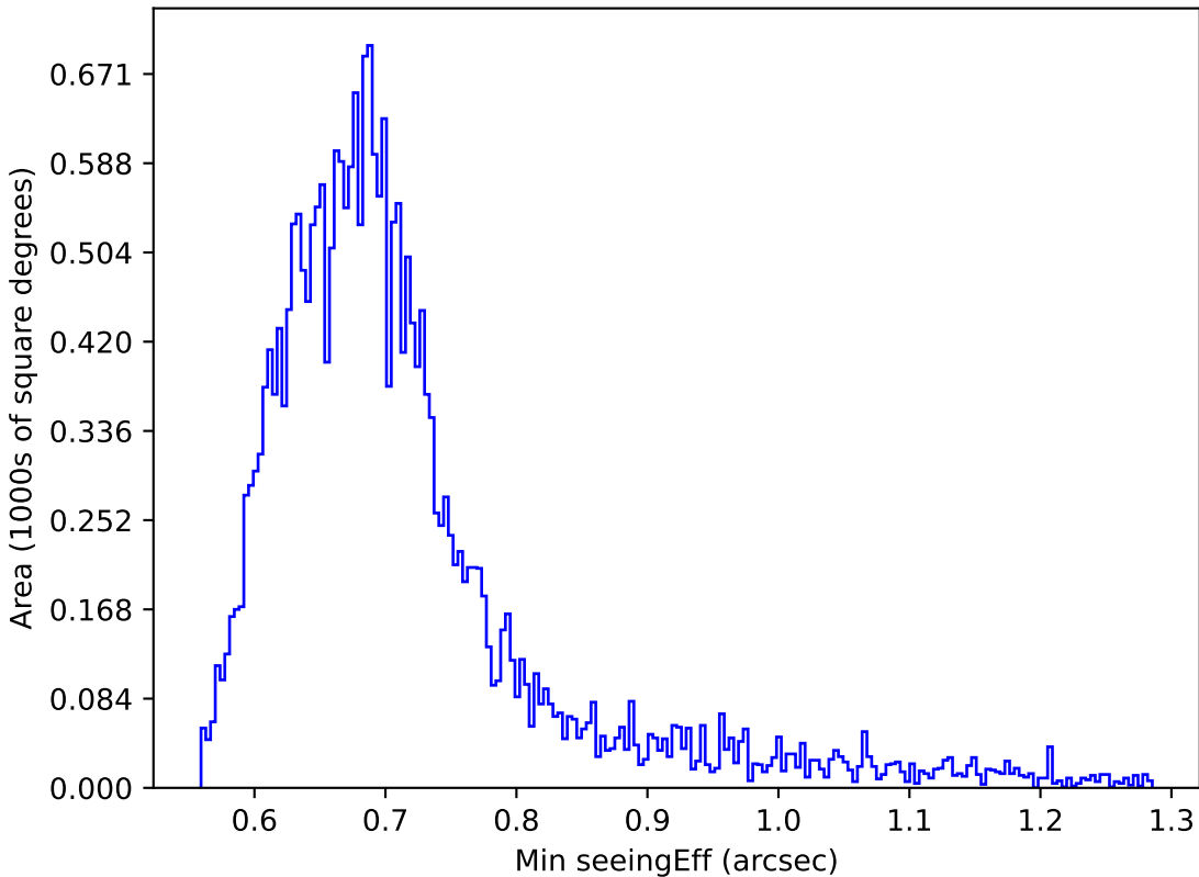
too_elab_r8_d2_giz_v3.4_10yrs Yr 1 r band: Min seeingEff
