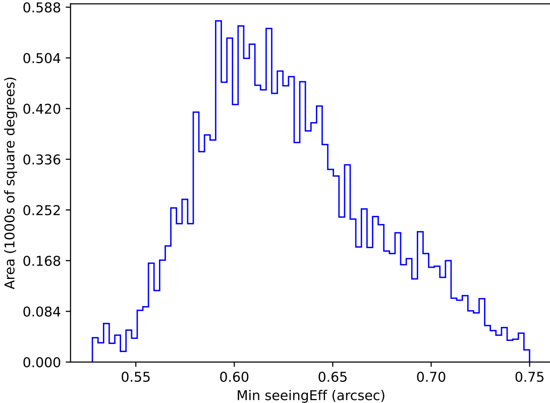
too_elab_r8_d2_giz_v3.4_10yrs WFD y band: Min seeingEff
