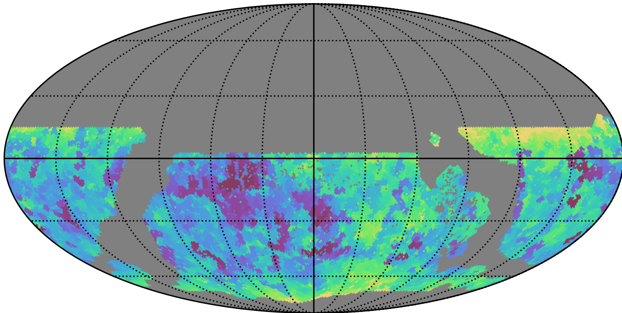
too_elab_r8_d2_giz_v3.4_10yrs WFD r band: Min seeingEff
