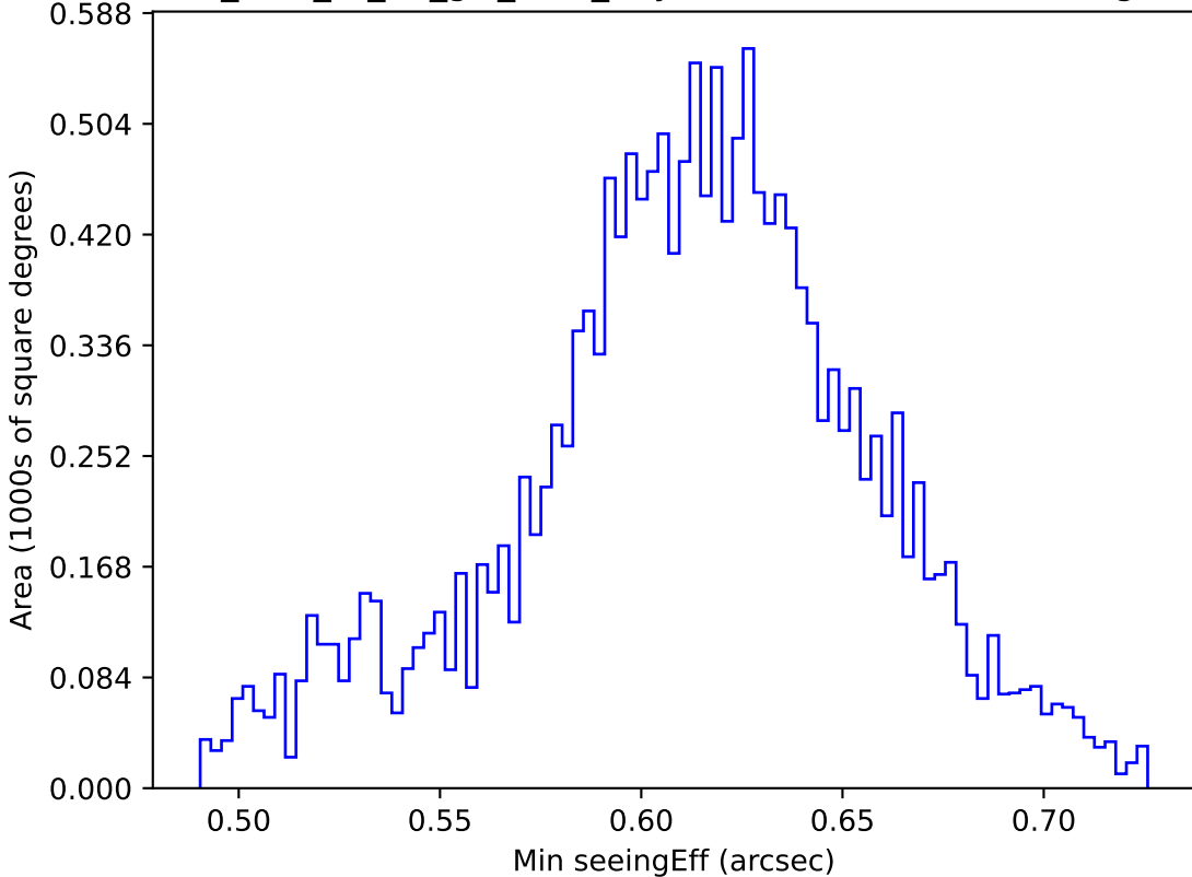
too_elab_r8_d2_giz_v3.4_10yrs WFD r band: Min seeingEff
