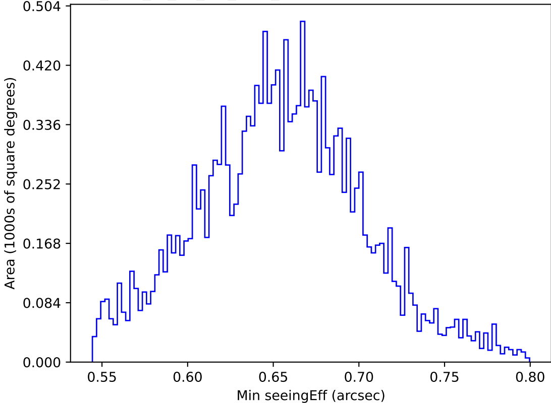
too_elab_r8_d2_giz_v3.4_10yrs WFD g band: Min seeingEff
