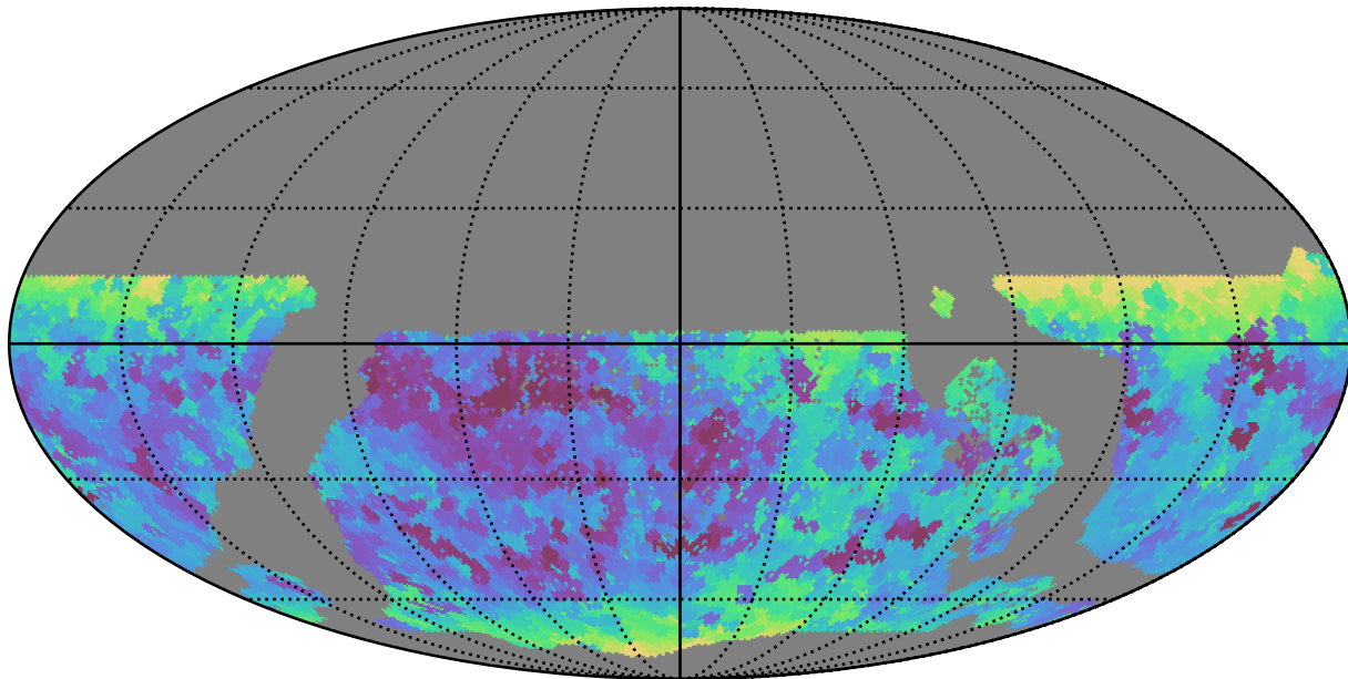
too_elab_r8_d2_giz_v3.4_10yrs WFD all bands: Min seeingEff
