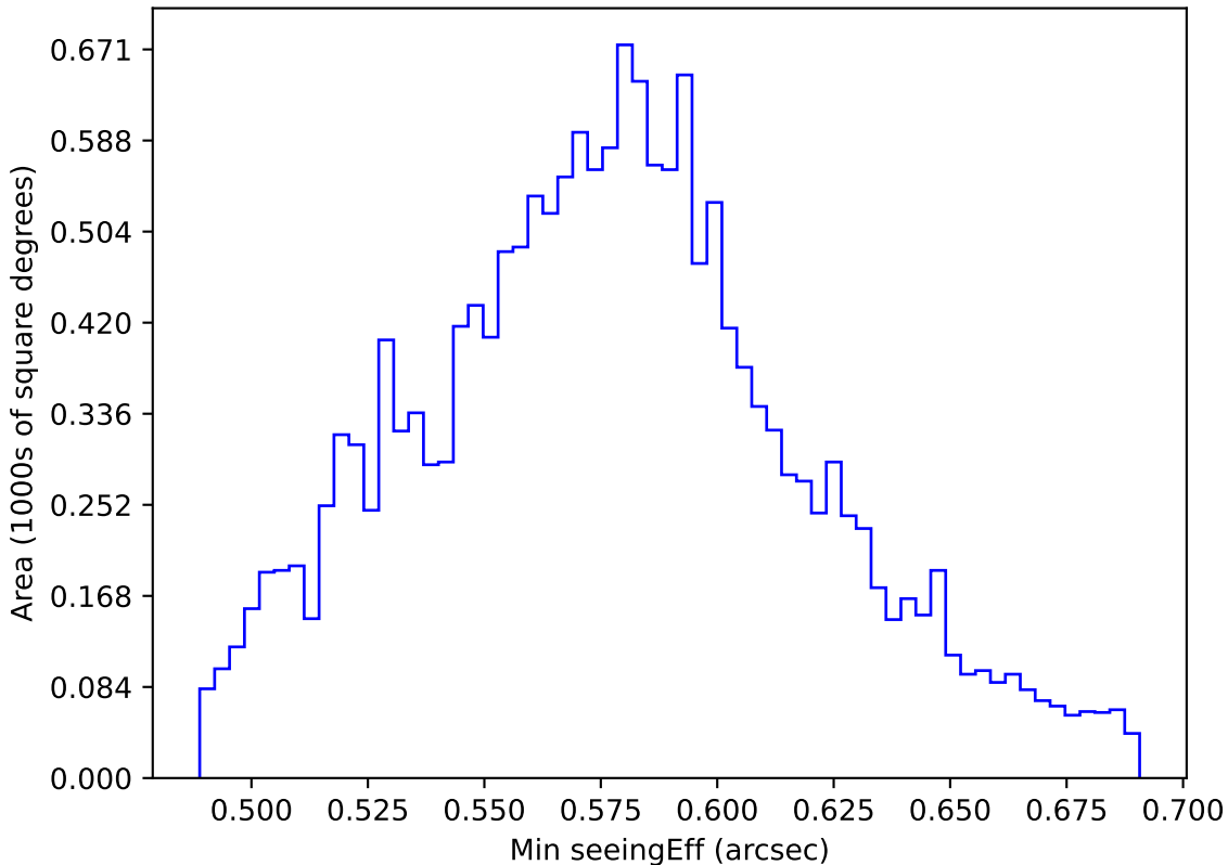
too_elab_r8_d2_giz_v3.4_10yrs WFD all bands: Min seeingEff
