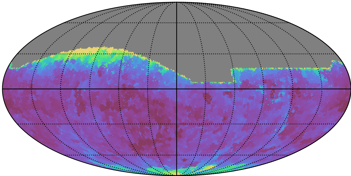
too_elab_r8_d2_giz_v3.4_10yrs All sky g band: Min seeingEff
