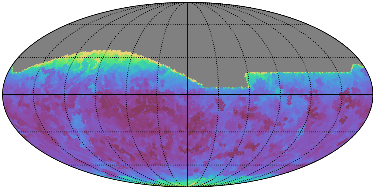
too_elab_r8_d2_giz_v3.4_10yrs All sky all bands: Min seeingEff
