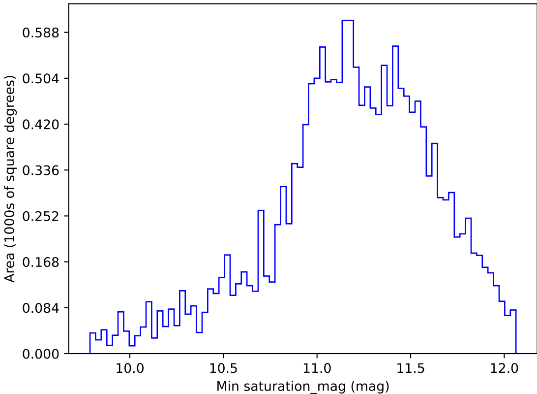
too_elab_r8_d2_giz_v3.4_10yrs WFD y band: Min saturation_mag
