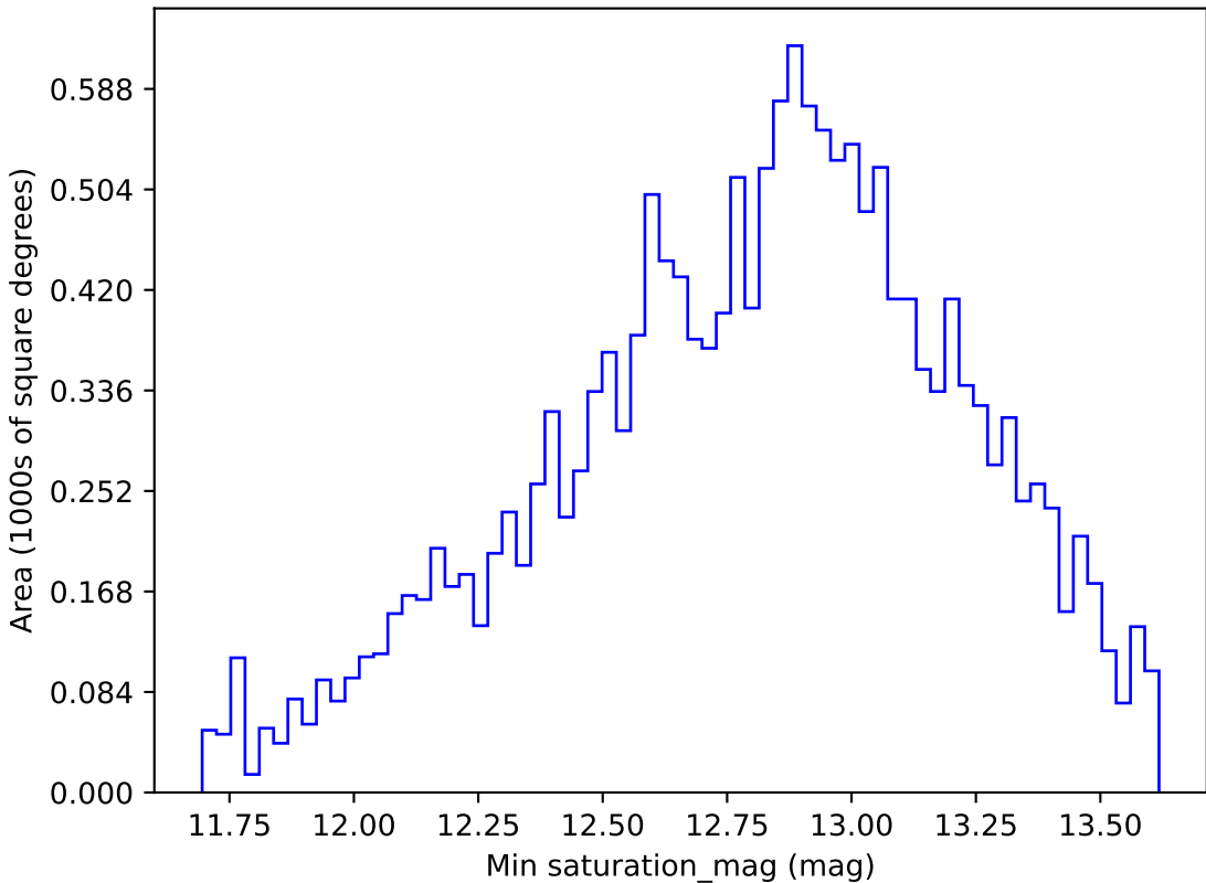
too_elab_r8_d2_giz_v3.4_10yrs WFD g band: Min saturation_mag
