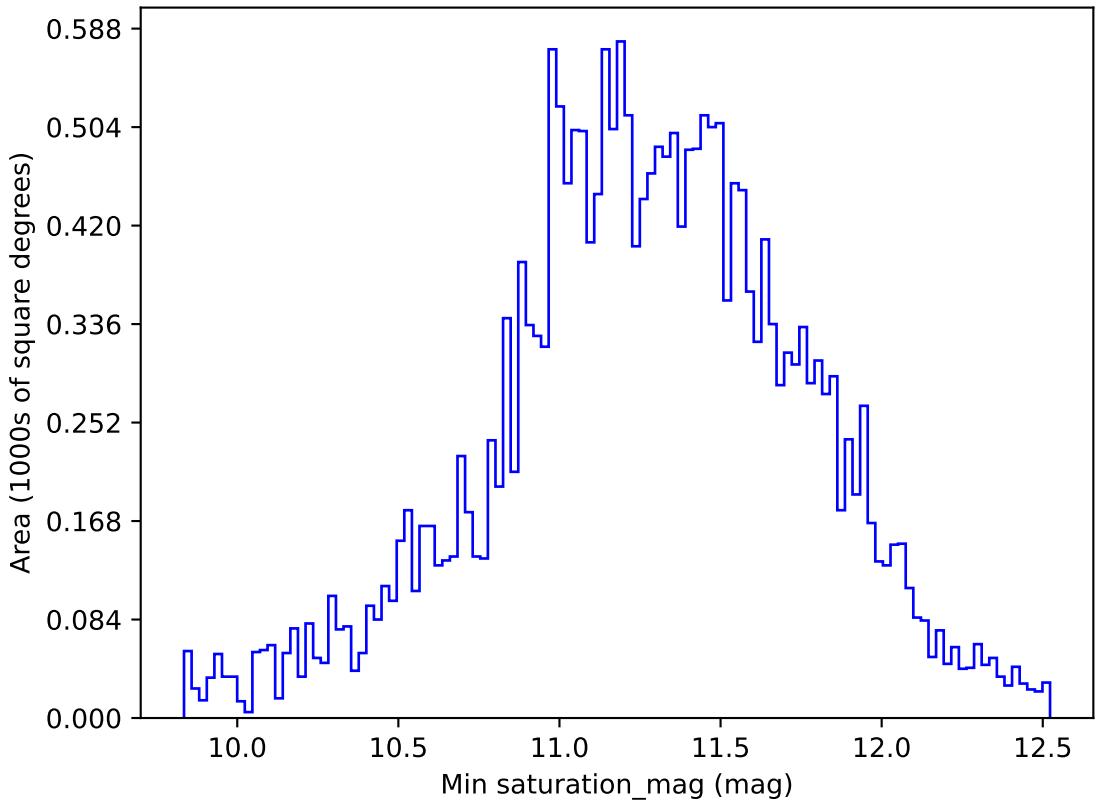
too_elab_r8_d2_giz_v3.4_10yrs All sky y band: Min saturation_mag
