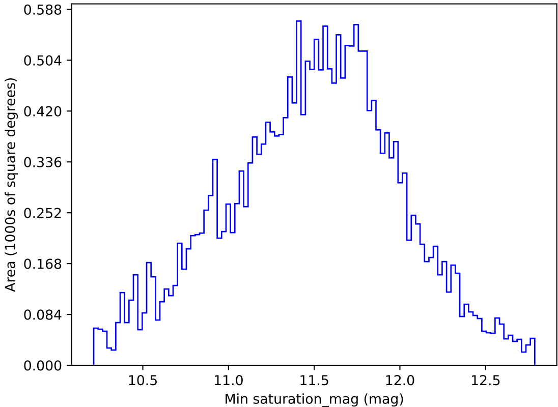
too_elab_r8_d2_giz_v3.4_10yrs All sky u band: Min saturation_mag
