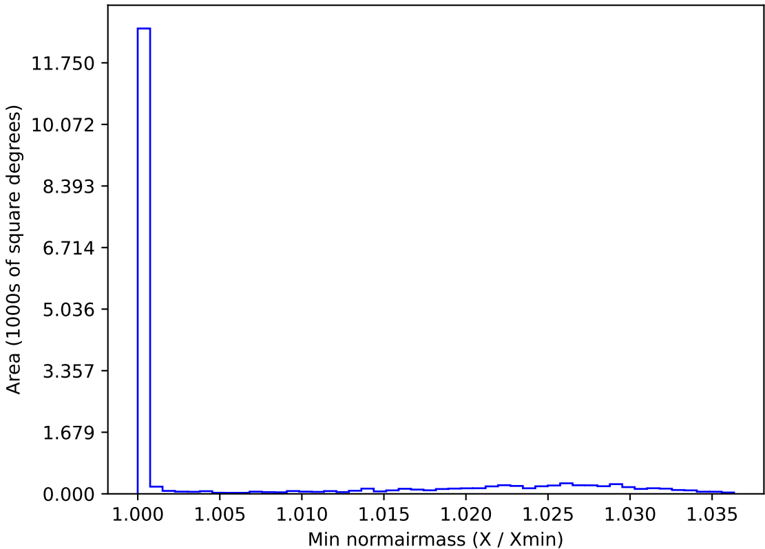
too_elab_r8_d2_giz_v3.4_10yrs WFD z band: Min normairmass
