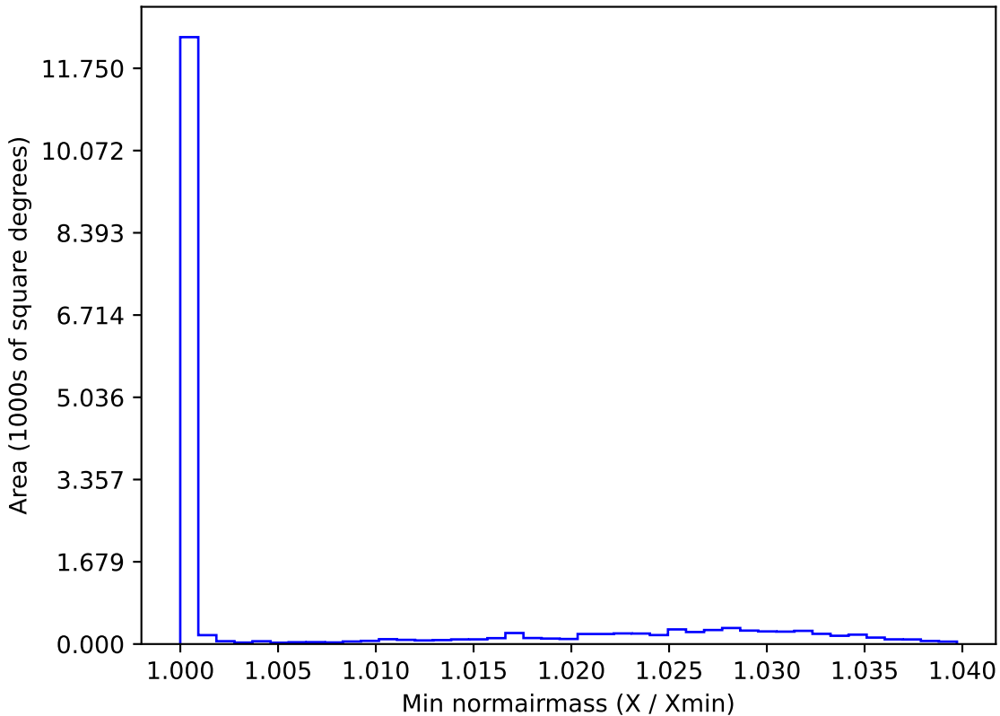
too_elab_r8_d2_giz_v3.4_10yrs WFD y band: Min normairmass
