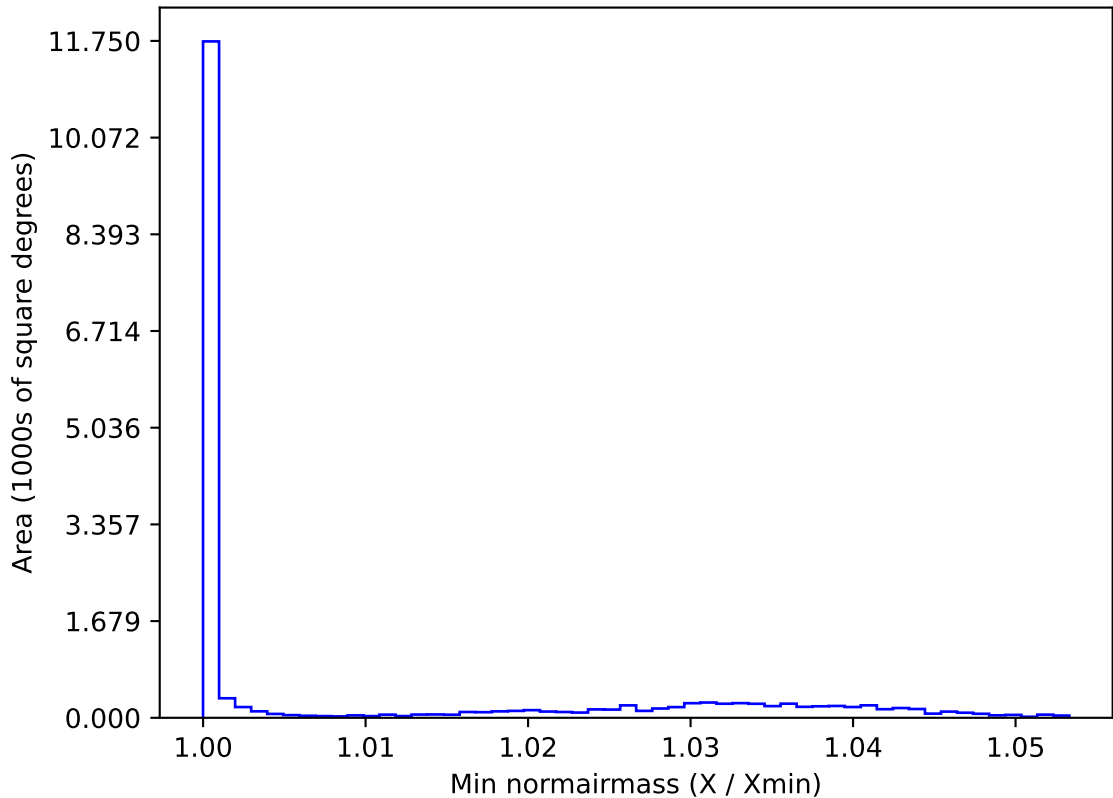
too_elab_r8_d2_giz_v3.4_10yrs WFD u band: Min normairmass
