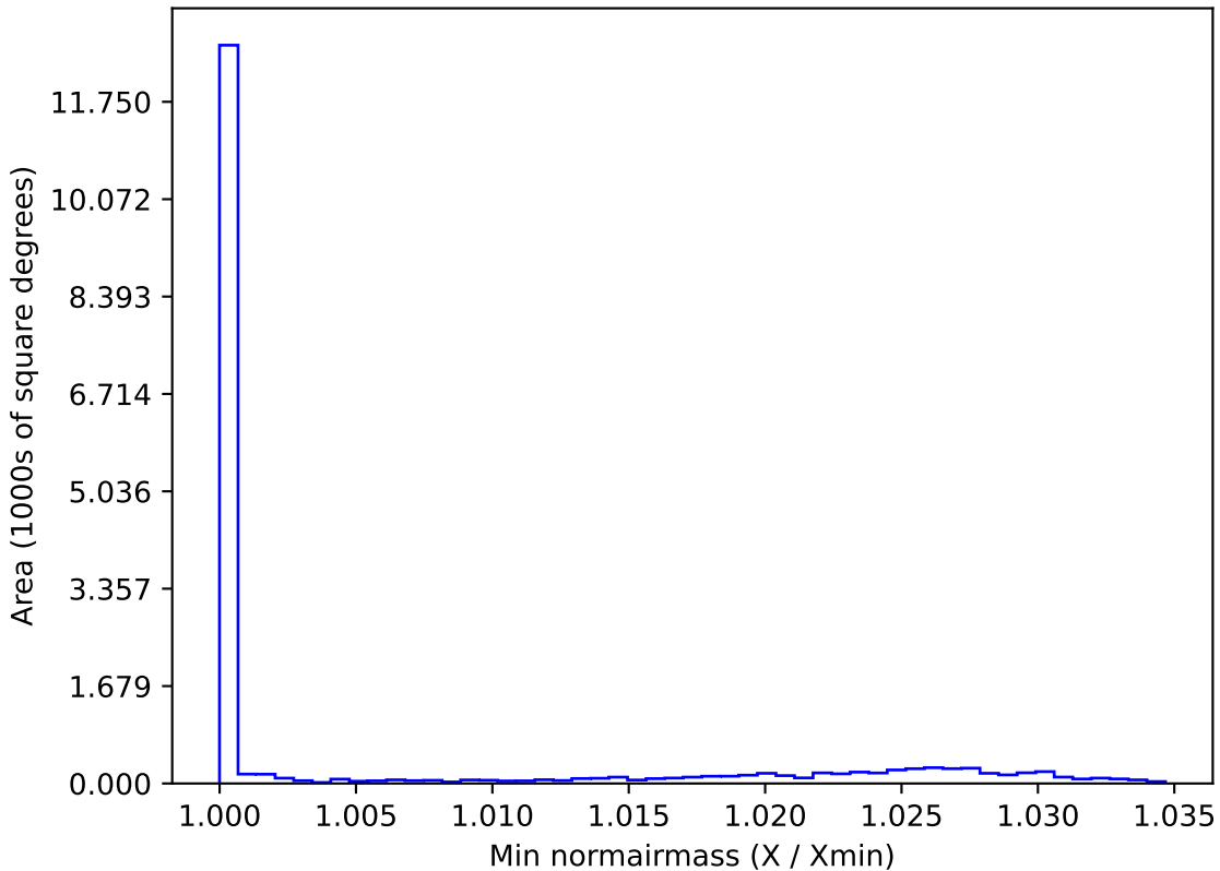
too_elab_r8_d2_giz_v3.4_10yrs WFD i band: Min normairmass
