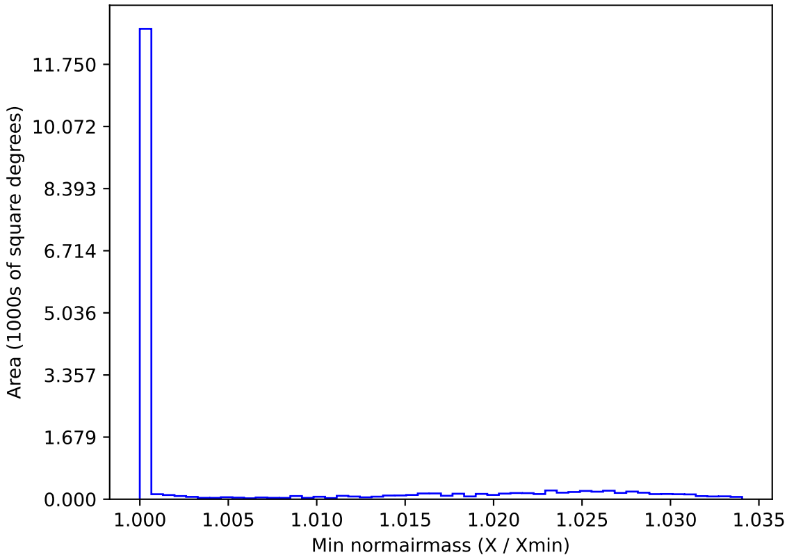
too_elab_r8_d2_giz_v3.4_10yrs WFD i band: Min normairmass
