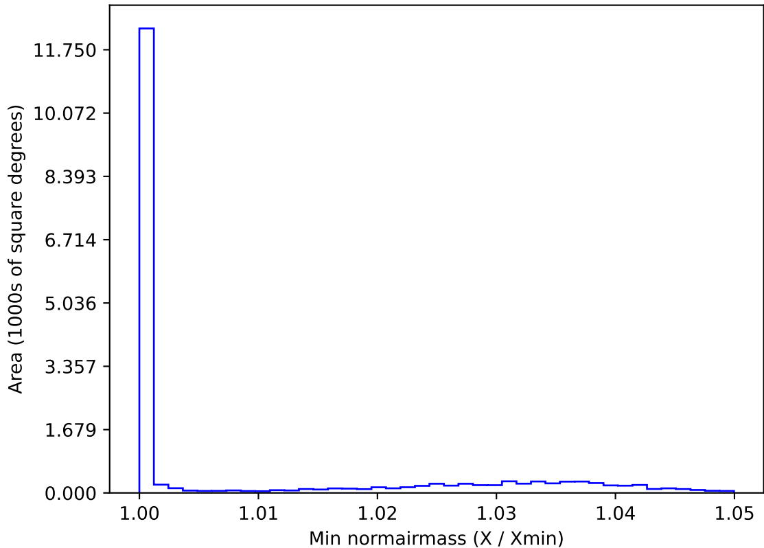
too_elab_r8_d2_giz_v3.4_10yrs WFD g band: Min normairmass
