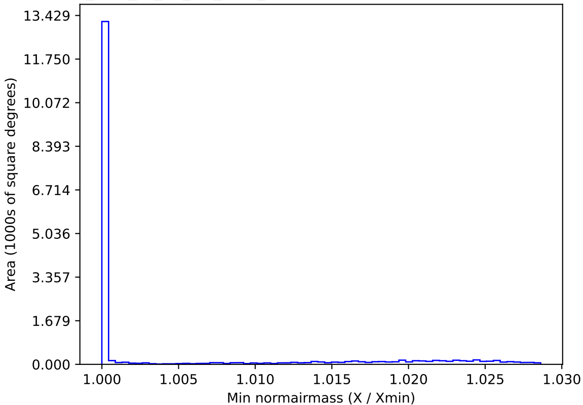
too_elab_r8_d2_giz_v3.4_10yrs WFD all bands: Min normairmass
