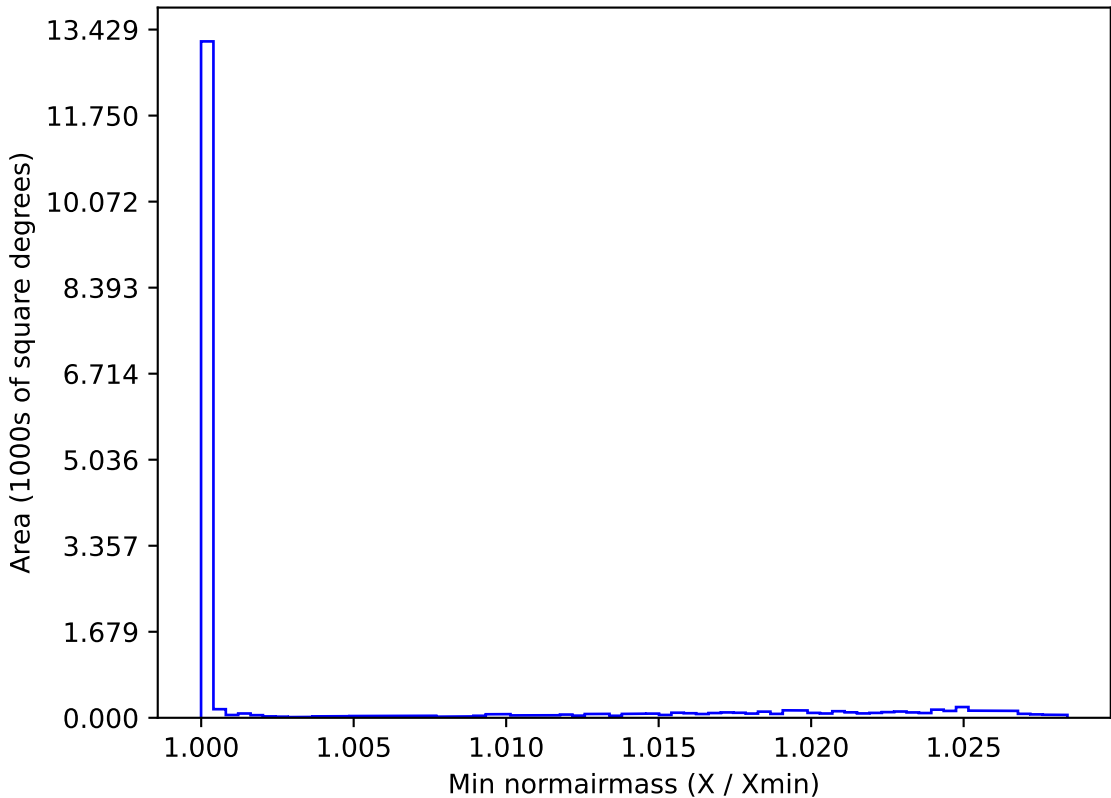
too_elab_r8_d2_giz_v3.4_10yrs WFD all bands: Min normairmass
