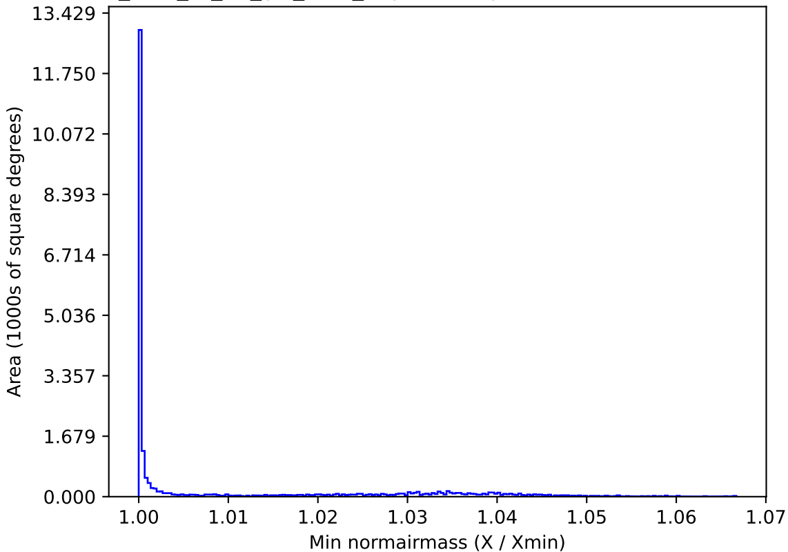
too_elab_r8_d2_giz_v3.4_10yrs All sky u band: Min normairmass
