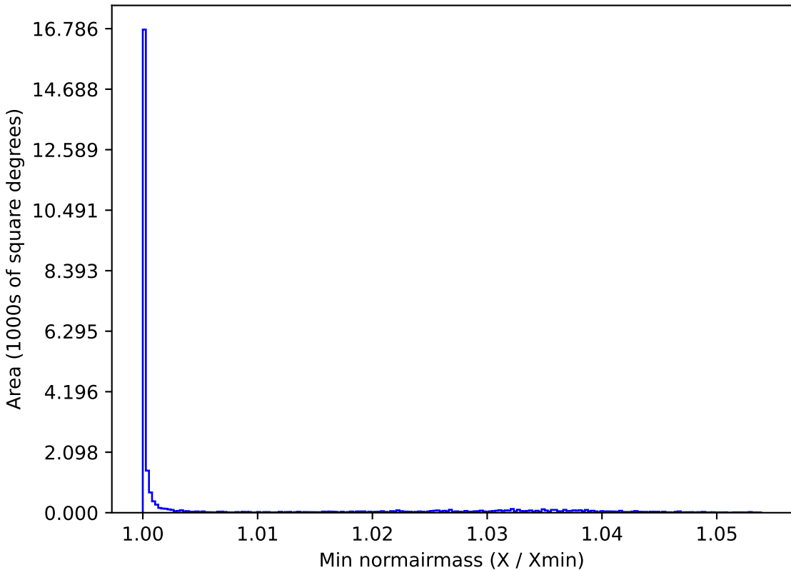
too_elab_r8_d2_giz_v3.4_10yrs All sky g band: Min normairmass
