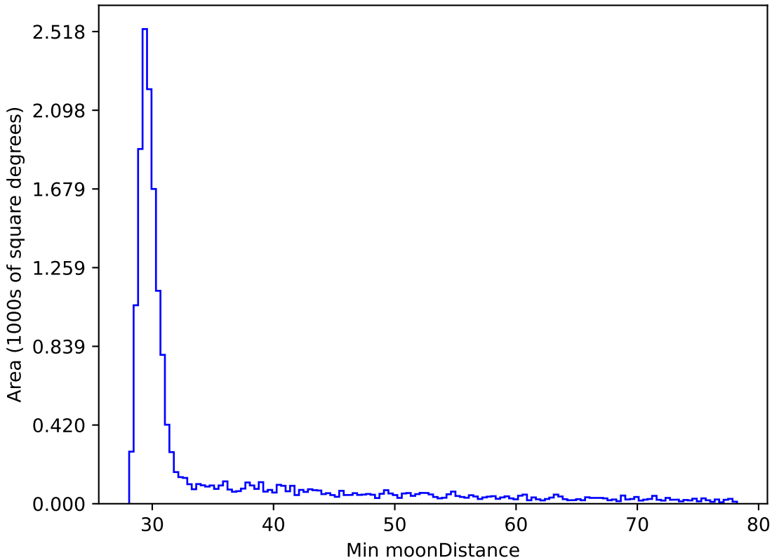
too_elab_r8_d2_giz_v3.4_10yrs WFD z band: Min moonDistance
