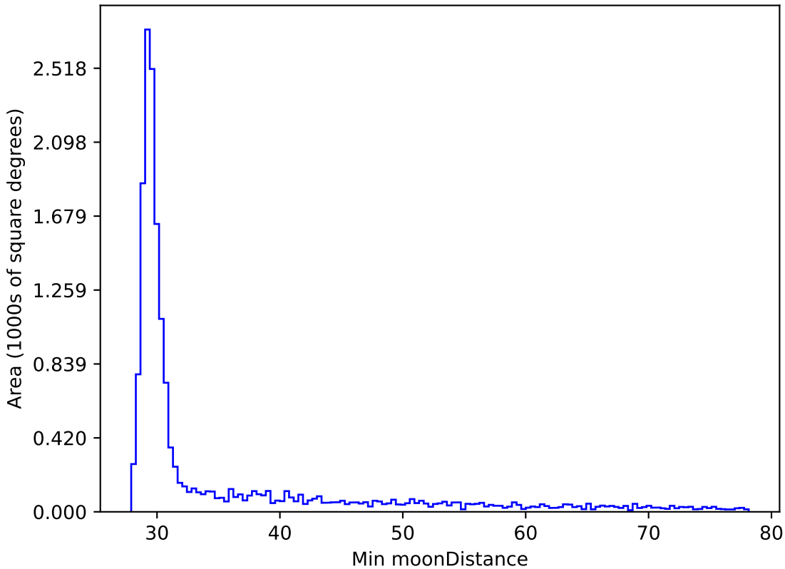
too_elab_r8_d2_giz_v3.4_10yrs WFD y band: Min moonDistance
