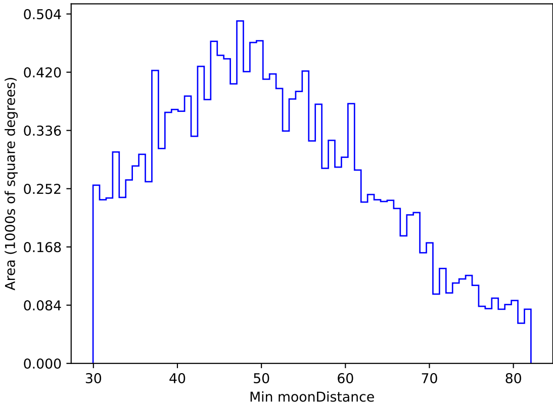
too_elab_r8_d2_giz_v3.4_10yrs WFD u band: Min moonDistance
