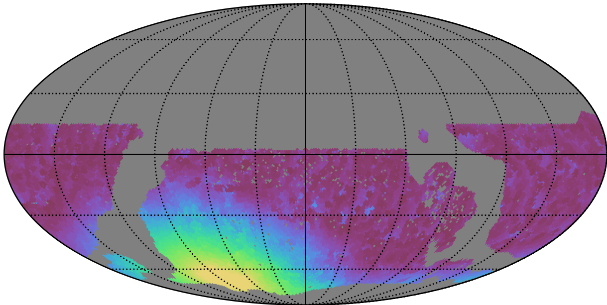
too_elab_r8_d2_giz_v3.4_10yrs WFD r band: Min moonDistance
