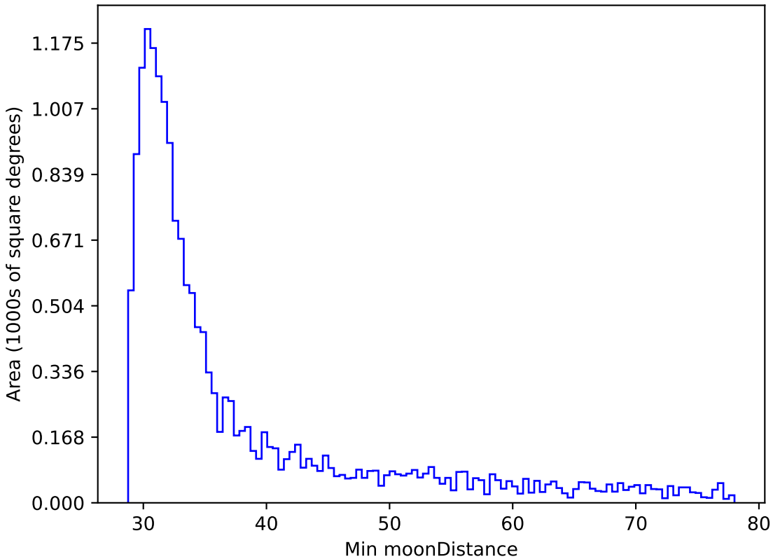
too_elab_r8_d2_giz_v3.4_10yrs WFD r band: Min moonDistance
