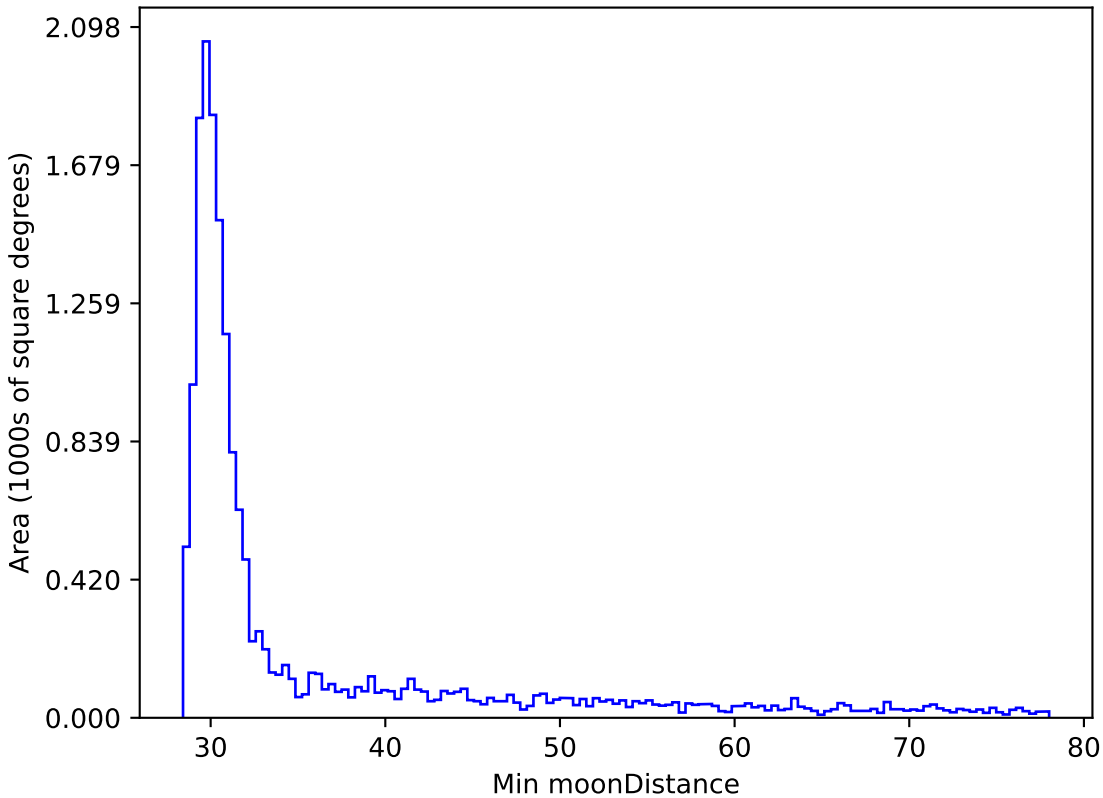
too_elab_r8_d2_giz_v3.4_10yrs WFD i band: Min moonDistance
