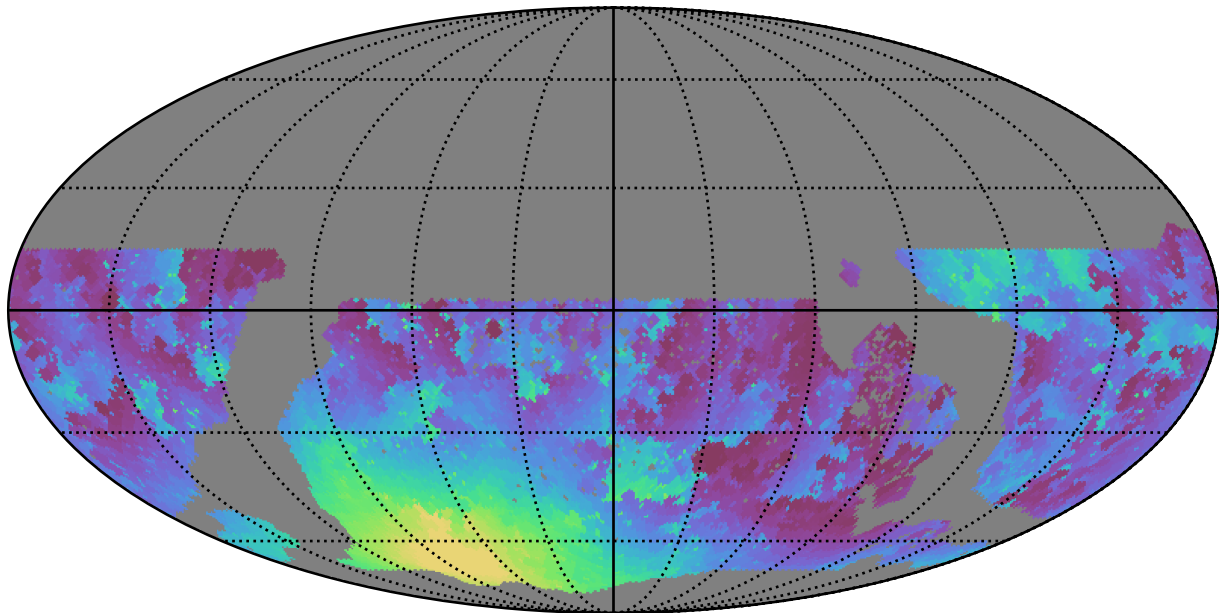
too_elab_r8_d2_giz_v3.4_10yrs WFD g band: Min moonDistance
