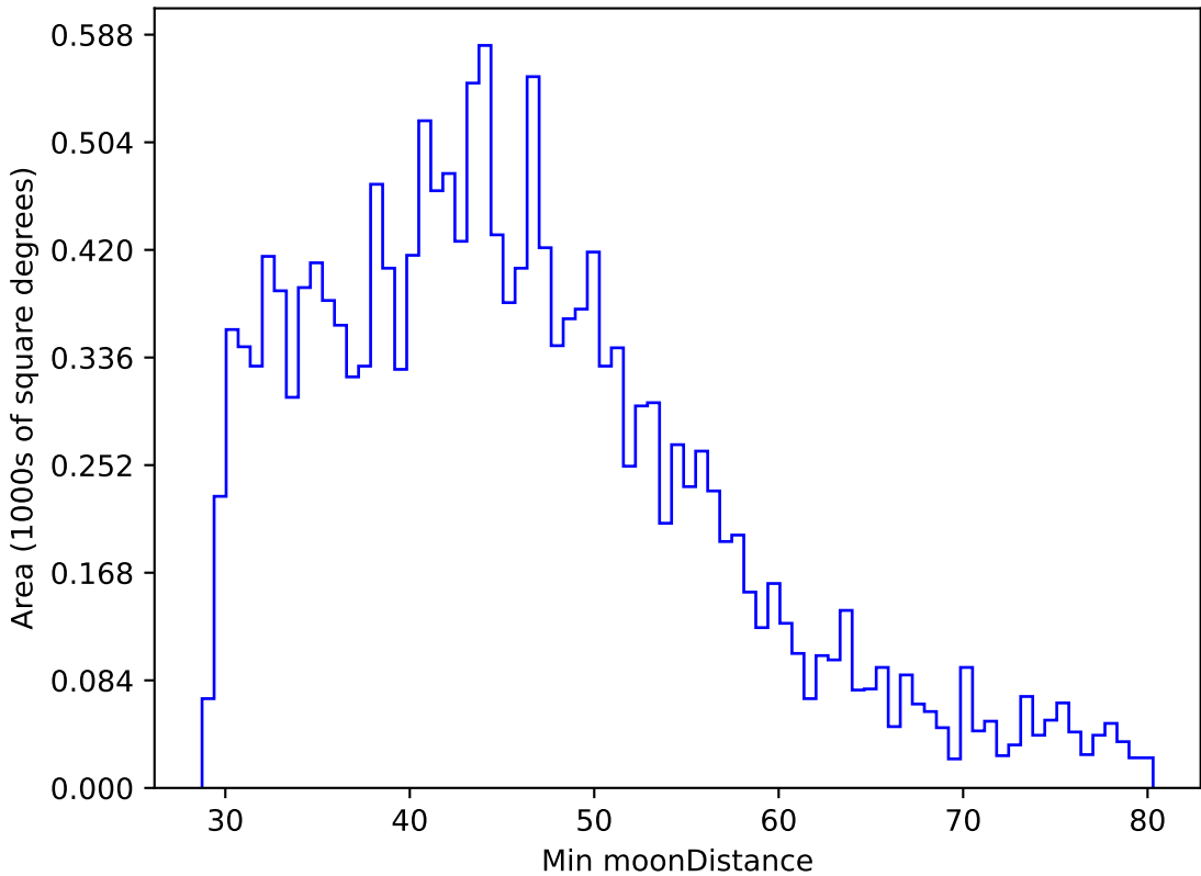
too_elab_r8_d2_giz_v3.4_10yrs WFD g band: Min moonDistance
