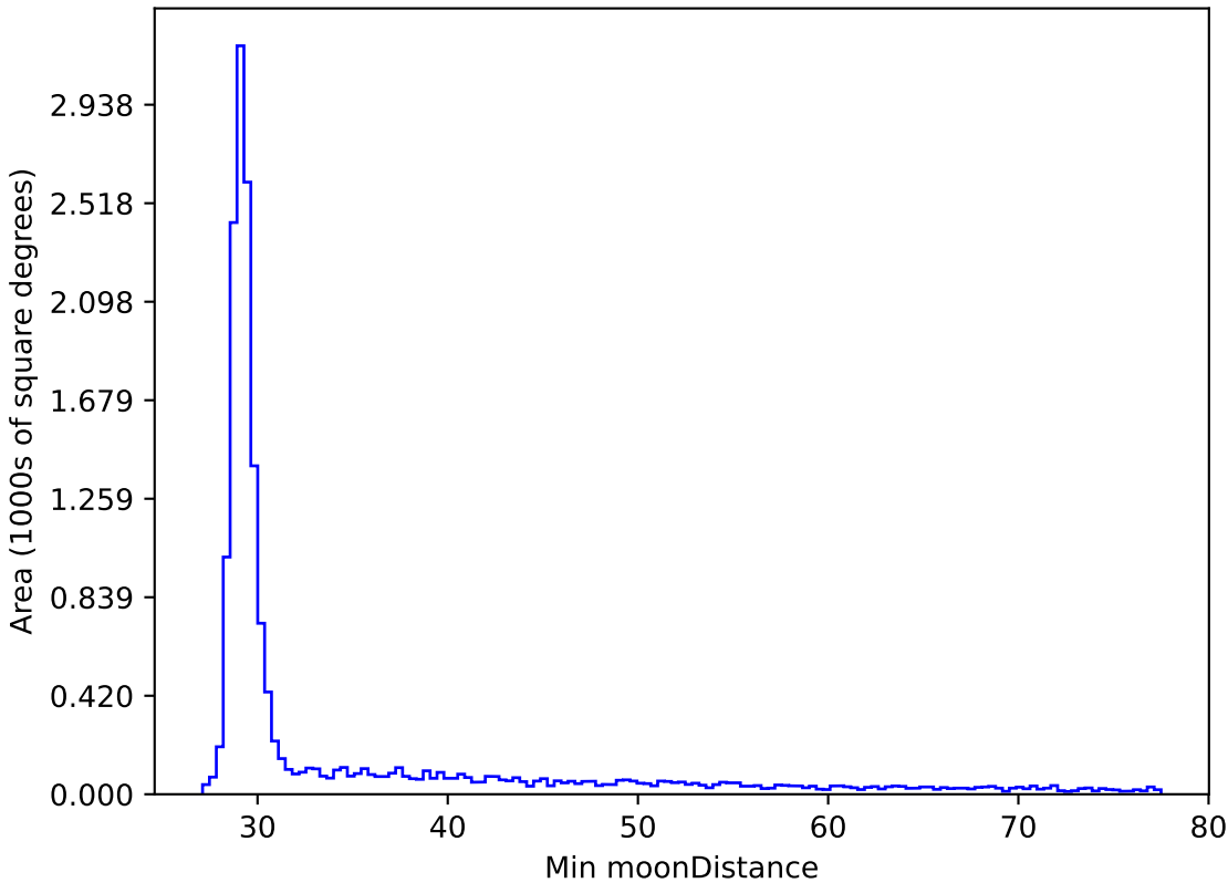
too_elab_r8_d2_giz_v3.4_10yrs WFD all bands: Min moonDistance
