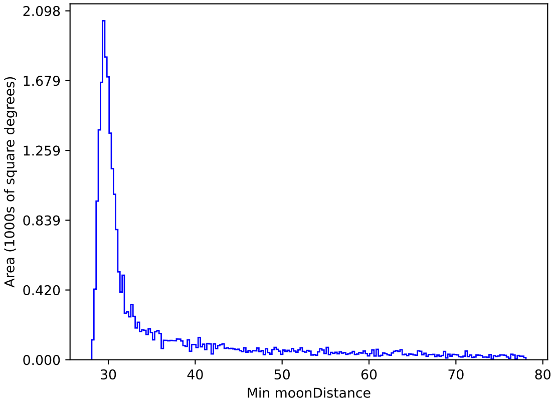
too_elab_r8_d2_giz_v3.4_10yrs All sky z band: Min moonDistance
