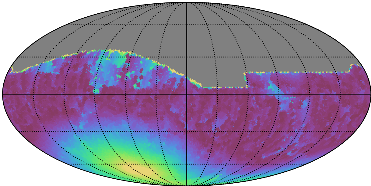
too_elab_r8_d2_giz_v3.4_10yrs All sky r band: Min moonDistance
