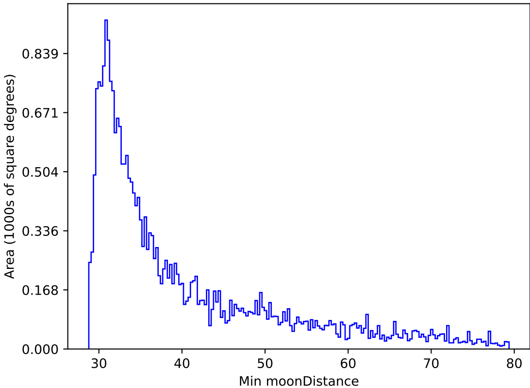
too_elab_r8_d2_giz_v3.4_10yrs All sky r band: Min moonDistance
