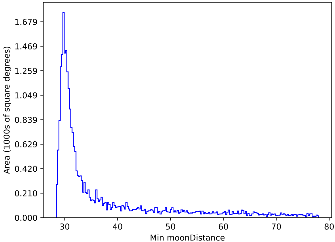
too_elab_r8_d2_giz_v3.4_10yrs All sky i band: Min moonDistance
