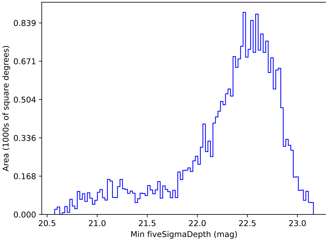
too_elab_r8_d2_giz_v3.4_10yrs Yr 1 z band: Min fiveSigmaDepth
