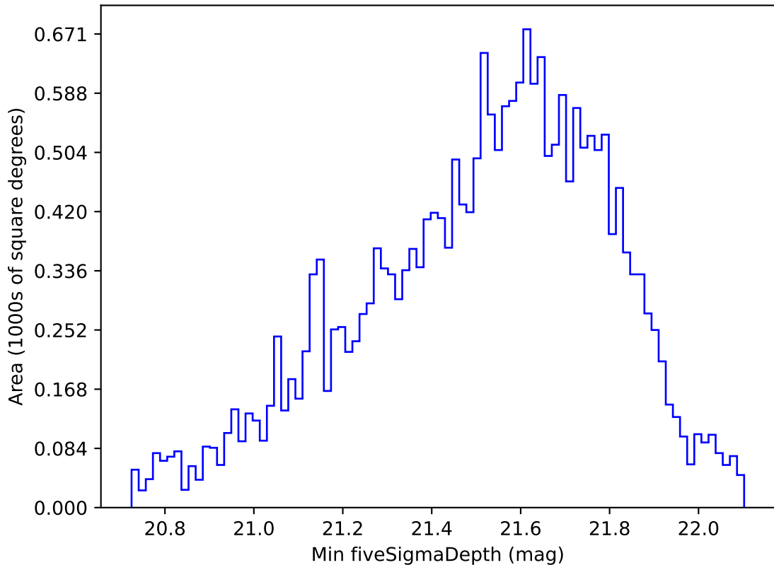
too_elab_r8_d2_giz_v3.4_10yrs Yr 1 y band: Min fiveSigmaDepth
