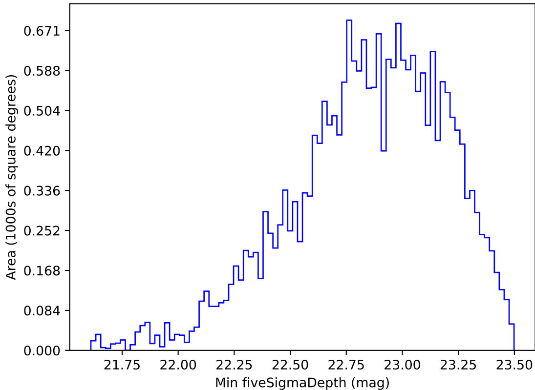
too_elab_r8_d2_giz_v3.4_10yrs Yr 1 u band: Min fiveSigmaDepth
