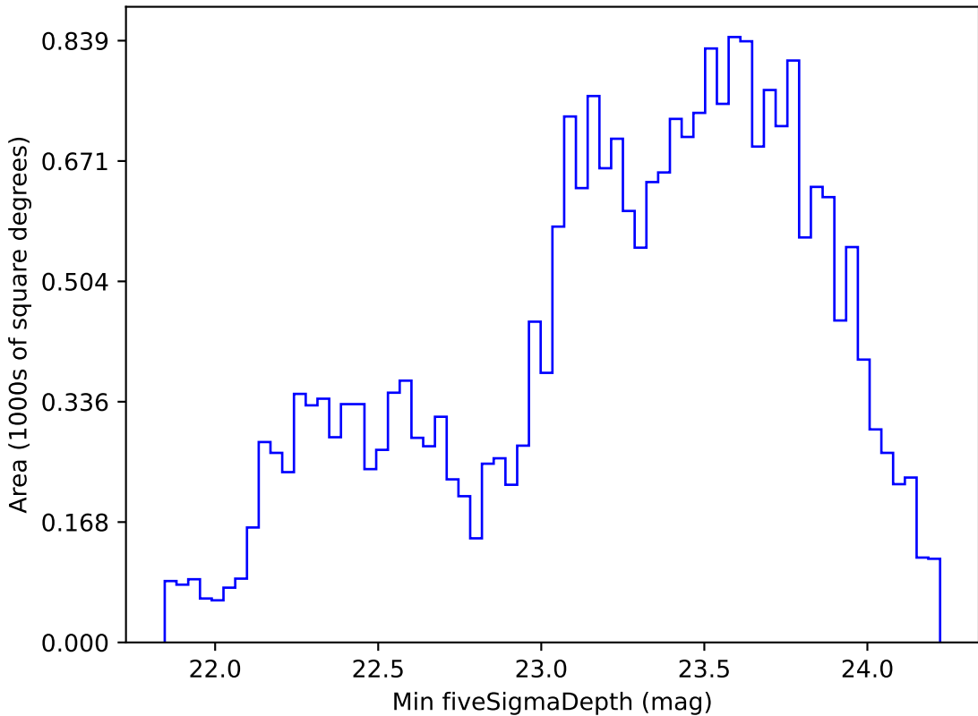
too_elab_r8_d2_giz_v3.4_10yrs Yr 1 r band: Min fiveSigmaDepth
