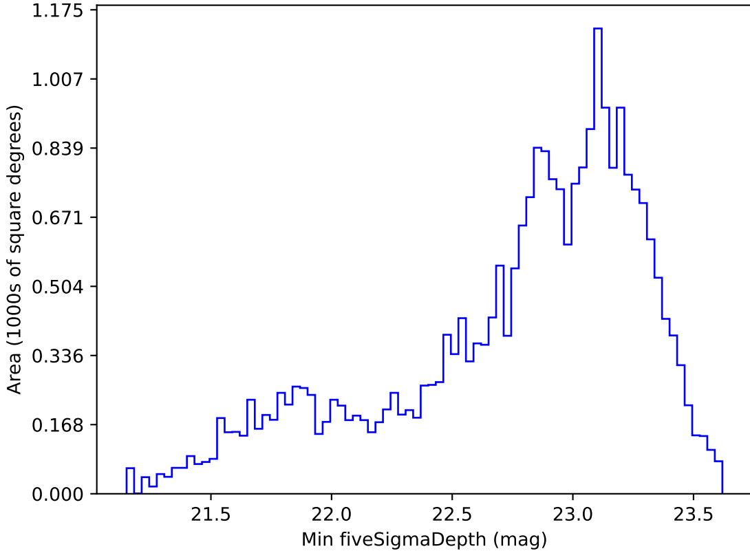
too_elab_r8_d2_giz_v3.4_10yrs Yr 1 i band: Min fiveSigmaDepth
