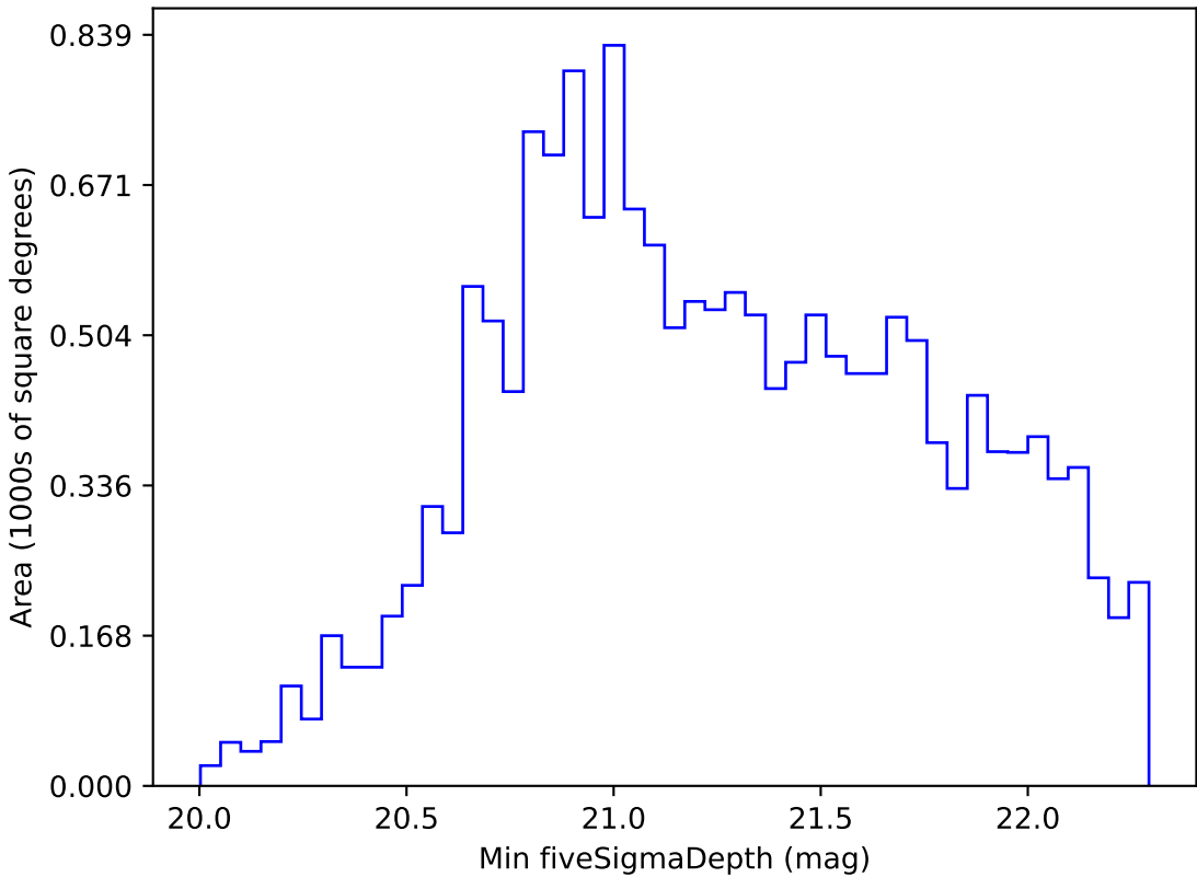
too_elab_r8_d2_giz_v3.4_10yrs WFD z band: Min fiveSigmaDepth
