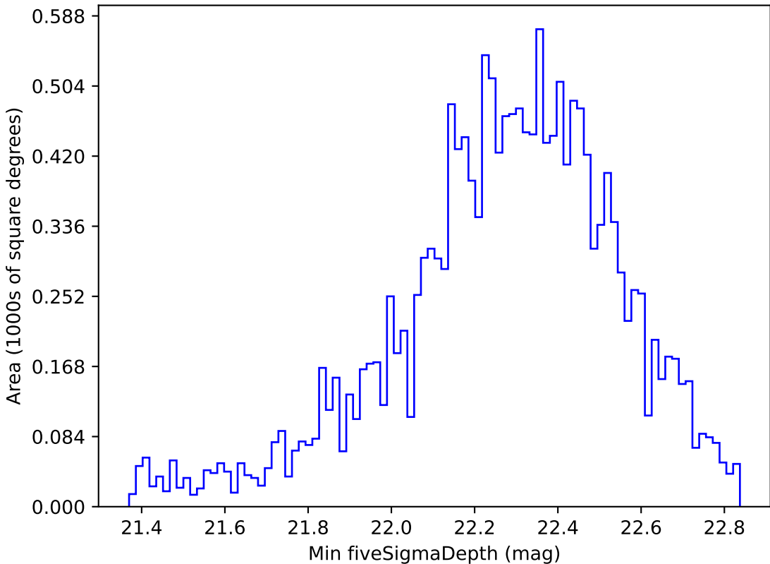
too_elab_r8_d2_giz_v3.4_10yrs WFD u band: Min fiveSigmaDepth
