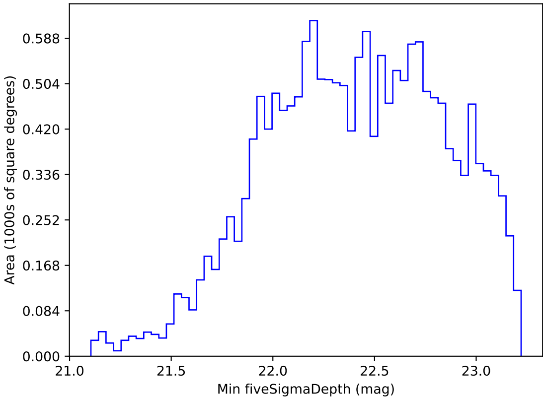
too_elab_r8_d2_giz_v3.4_10yrs WFD r band: Min fiveSigmaDepth
