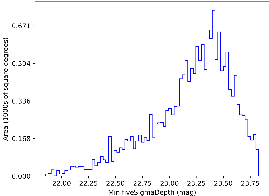
too_elab_r8_d2_giz_v3.4_10yrs WFD g band: Min fiveSigmaDepth
