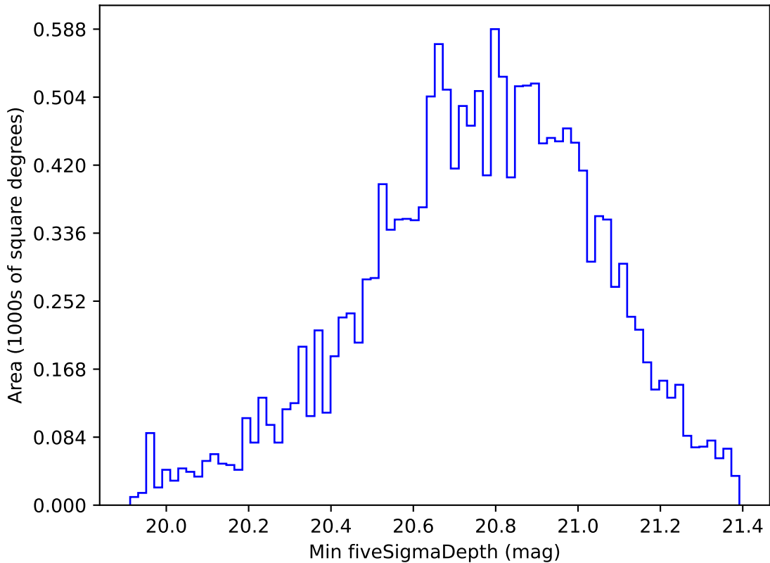
too_elab_r8_d2_giz_v3.4_10yrs WFD all bands: Min fiveSigmaDepth
