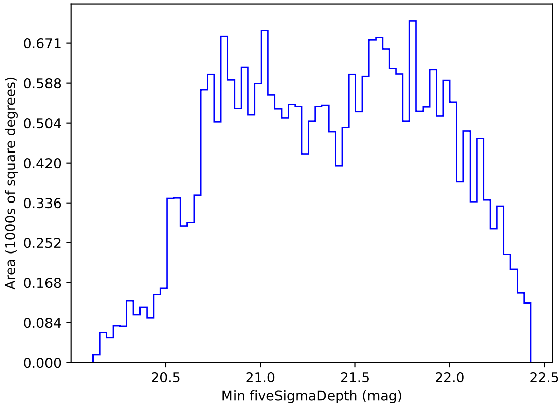
too_elab_r8_d2_giz_v3.4_10yrs All sky z band: Min fiveSigmaDepth
