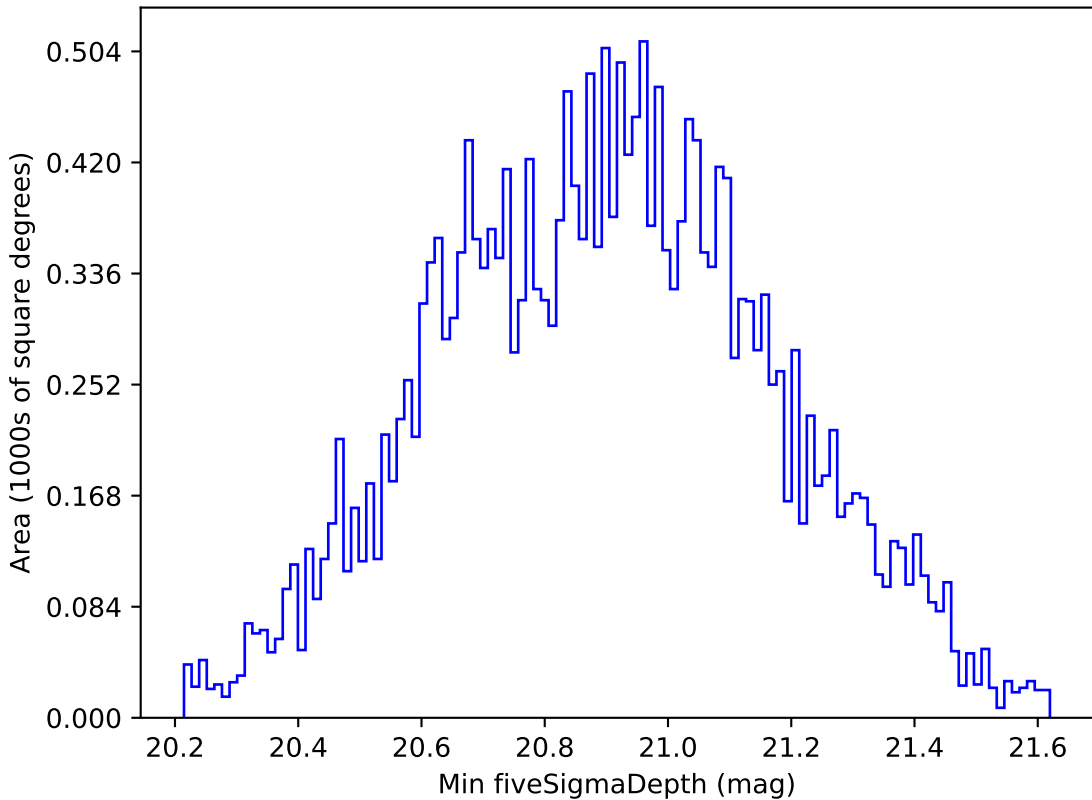
too_elab_r8_d2_giz_v3.4_10yrs All sky y band: Min fiveSigmaDepth
