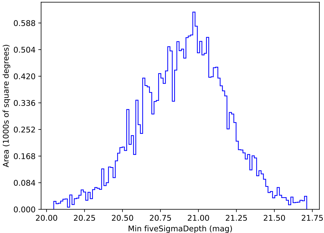
too_elab_r8_d2_giz_v3.4_10yrs All sky y band: Min fiveSigmaDepth
