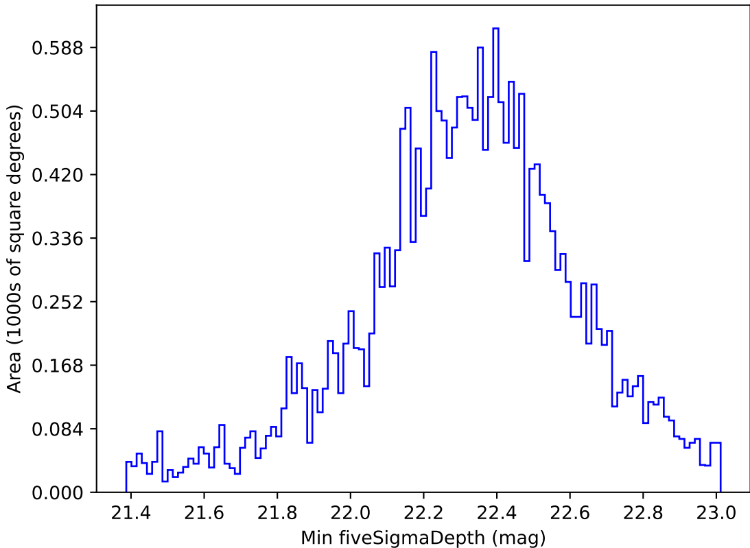
too_elab_r8_d2_giz_v3.4_10yrs All sky u band: Min fiveSigmaDepth
