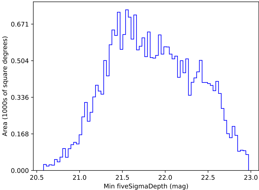
too_elab_r8_d2_giz_v3.4_10yrs All sky i band: Min fiveSigmaDepth
