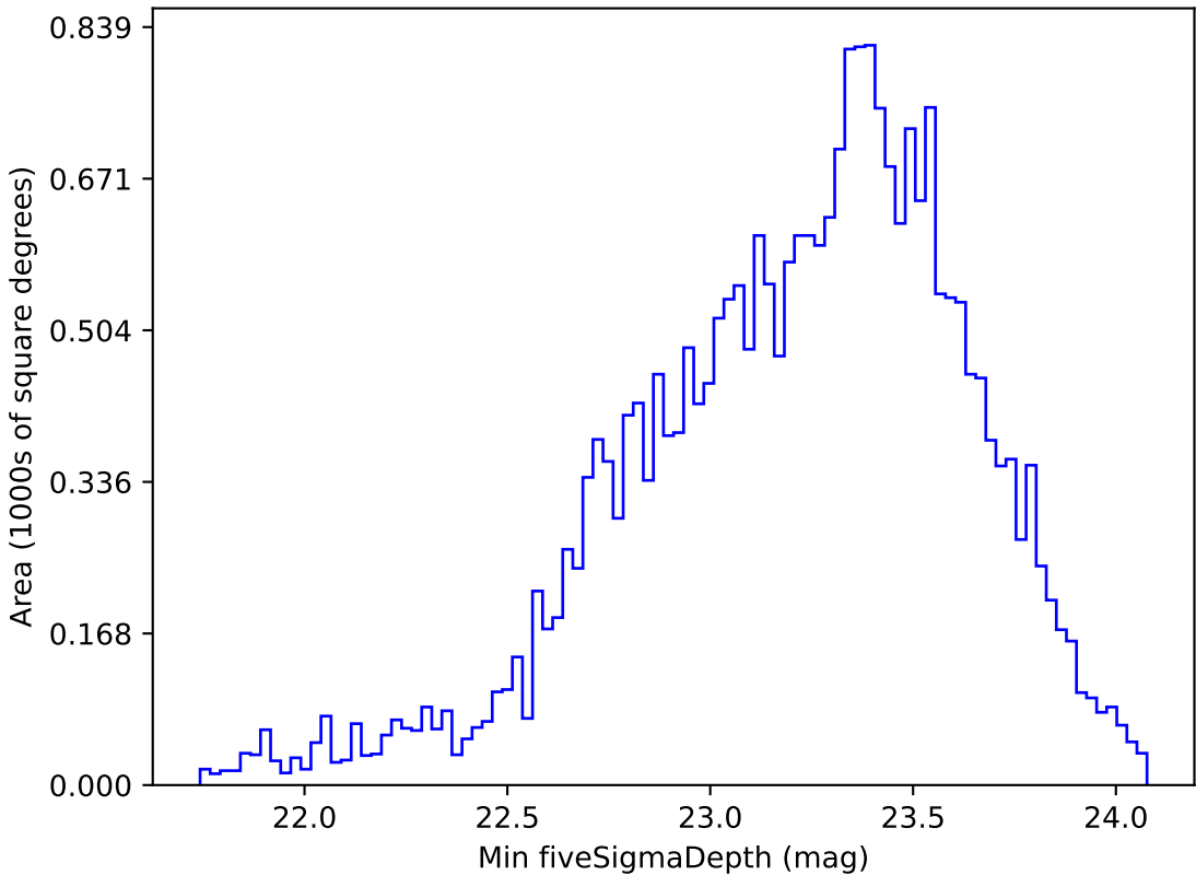
too_elab_r8_d2_giz_v3.4_10yrs All sky g band: Min fiveSigmaDepth
